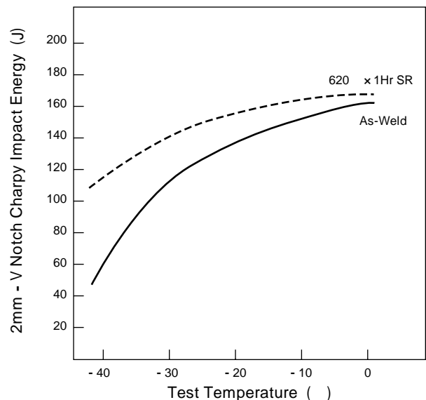
Fig. 2 - Typical Impact Energy of LB-52-18 Deposited Metal
